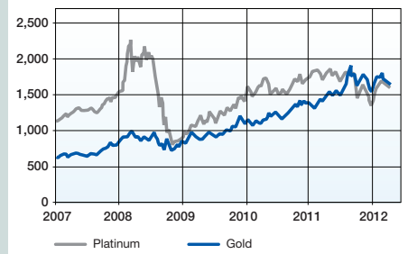
Figure 5: Gold vs Platinum US$/oz
